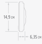
In-dash Mount
